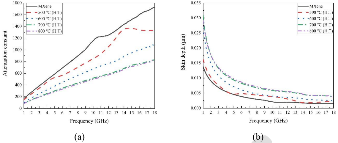
Fig. 7. The changes in a) attenuation constant and b) skin depth in relation to frequency (within 1-18 GHz) for \text{Ti}_3\text{C}_2\text{T}_x MXene phase before and after annealing process at different annealing temperatures.
